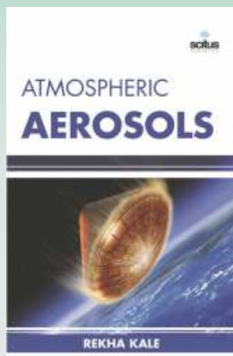
Atmospheric Aerosols
