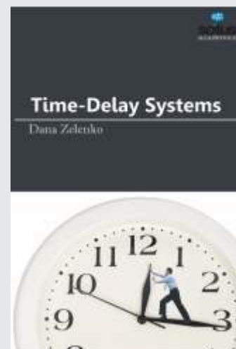
Time-Delay Systems
