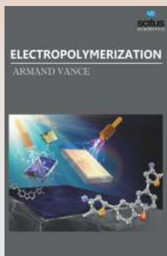
Electropolymerization
