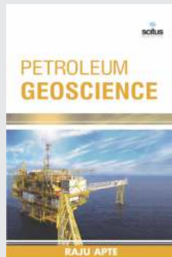
Petroleum Geoscience
