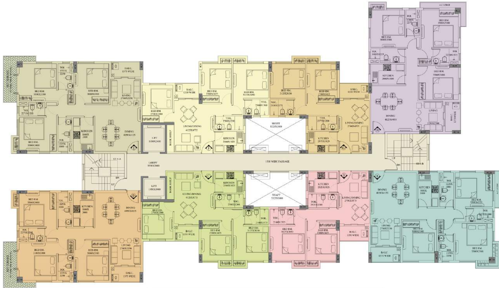
AREA STATEMENT-4TH FLOOR-TOWER-4
