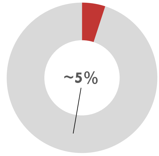
Vinyl Sulphone
